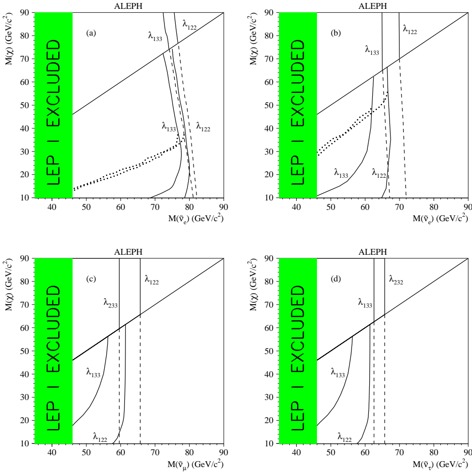
Fig. 10a–d. The 95% C.L. limits in the (m_\chi, m_{\tilde{\nu}}) plane at \tan\beta = 2 . Above the diagonal line the lightest neutralino is heavier than the sneutrinos, and only the direct decays are allowed. Below the line the indirect decays generally dominate, but the branching ratio of the direct (dashed lines) to indirect (full lines) decays depends on the magnitude of the coupling \lambda_{ijk} . The two choices of \lambda_{122} and \lambda_{133} correspond to the best and worst case exclusions for the indirect decays. a and b show the electron-sneutrino limit in the gaugino region ( \mu = -200 \text{ GeV}/c ) and the higgsino region ( M_2 = 400 \text{ GeV}/c^2 ), respectively, assuming \text{BR}(\tilde{\nu}_e \rightarrow \nu_e \chi) = 100\% for the indirect decays (full lines), and conservatively assuming zero efficiency for the cascade decays (dotted lines). c and d show the mass limits on muon- and tau-sneutrinos
