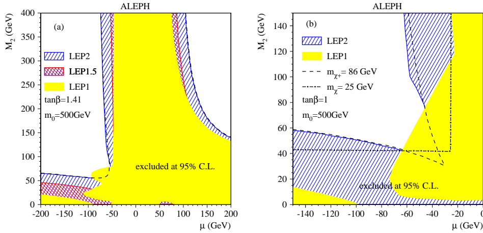
Fig. 4. Regions in the (\mu, M_2) plane excluded at 95% C.L. at m_0 = 500 \text{ GeV}/c^2 and a \tan\beta = 1.41 or b \tan\beta = 1 , assuming that the indirect decays dominate. The superimposed dashed and dash-dotted lines show the kinematic limit M_{\chi^+} = 86 \text{ GeV}/c^2 , and a fixed neutralino mass of M_{\chi} = 25 \text{ GeV}/c^2 . The neutralino limit of M_{\chi} = 25 \text{ GeV}/c^2 is set at \tan\beta = 1 and (\mu, M_2) \sim (-60, 40) by an interplay of the LEP1 and LEP2 exclusion limits
