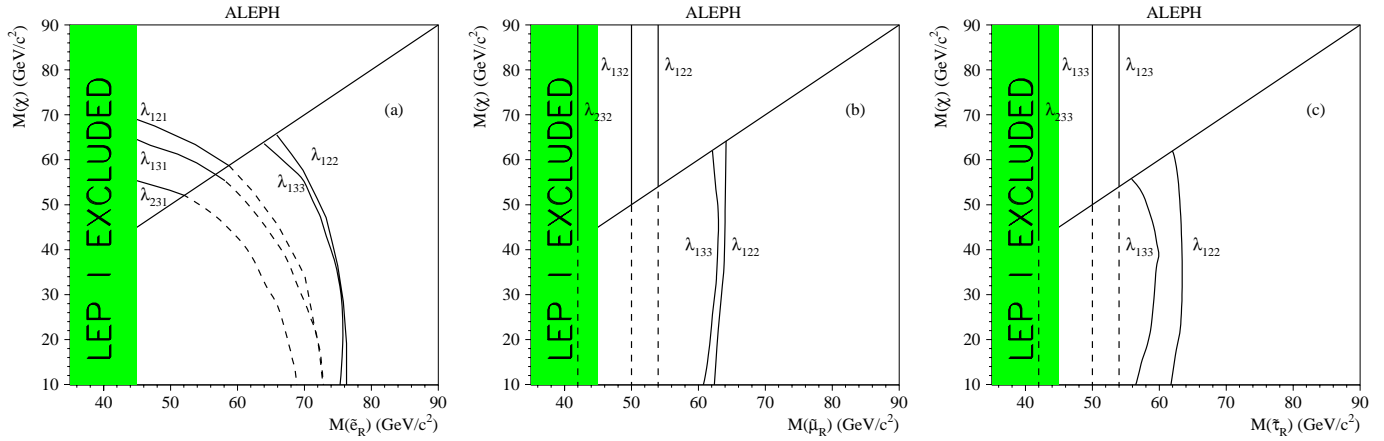
Fig. 8a–c. The 95% C.L. limits in the (m_\chi, m_{\tilde{l}_R}) plane at \tan\beta = 2 . Above the diagonal line the lightest neutralino is heavier than the sleptons, and only the direct decays are allowed. Below the line the indirect decays generally dominate, but the branching ratio of the direct (dashed lines) to indirect (full lines) decays depends on the magnitude of the coupling \lambda_{ijk} . The two choices of \lambda_{122} and \lambda_{133} correspond to the best and worst case exclusions for the indirect decays, respectively. a shows the selectron limit in the gaugino region for \mu = -200 \text{ GeV}/c^2 , b and c show the mass limits on smuons and staus
