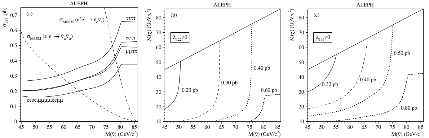
Fig. 9a–c. The 95% C.L. sneutrino exclusion cross sections scaled to \sqrt{s} = 172 \text{ GeV} . For the purpose of these plots a \beta^3/s cross section dependence, valid for scalar pair-production in the s -channel, was assumed. a shows \sigma_{\text{excluded}}^{172} for the direct decays of sneutrinos. Superimposed are the MSSM cross sections at \tan\beta = 2 for electron-sneutrino production ( M_2 = 100 \text{ GeV}/c^2 , \mu = -200 \text{ GeV}/c^2 ) and muon-sneutrino production. In this case the electron-sneutrino cross-section is used as an illustration of the potential gains due to the constructive interference. b and c show contours of \sigma_{\text{excluded}}^{172} for the indirect decays in the (M_\chi, M_{\tilde{\nu}}) plane for the best-case exclusion ( \lambda_{122} ) and the worst-case exclusion ( \lambda_{133} )
