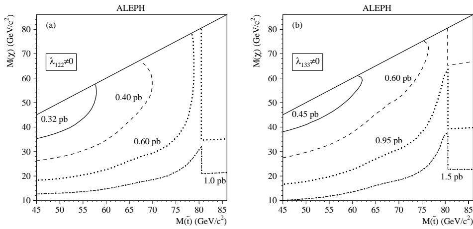
Fig. 11a,b. The 95% C.L. stop exclusion cross sections at \sqrt{s} = 172 GeV. a and b show contours of \sigma_{\text{excluded}}^{172} in the (M_\chi, M_{\bar{t}}) plane for the best-case exclusion ( \lambda_{122} ) and the worst-case exclusion ( \lambda_{133} )
