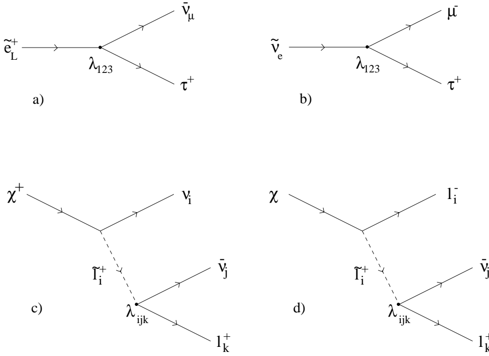
Fig. 1. Examples of R-parity violating decays of a left-handed selectrons, b electron-sneutrinos via the coupling \lambda_{123} , c charginos, d neutralinos via slepton exchange
