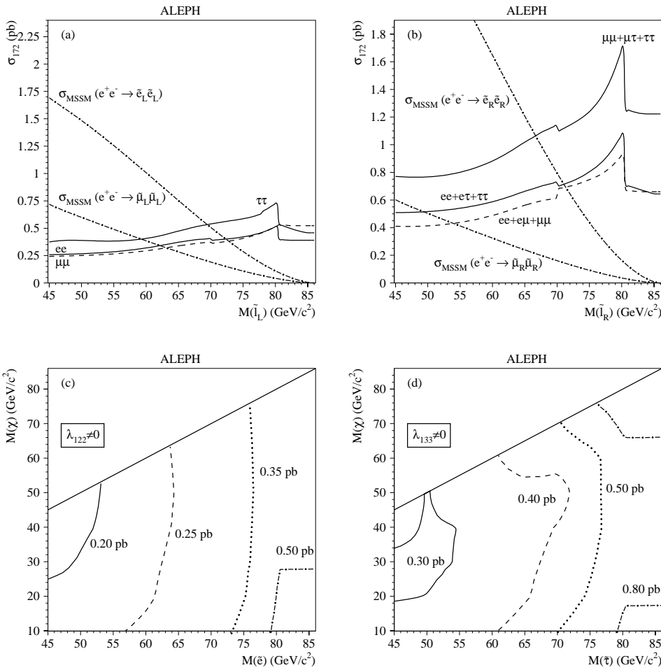
Fig. 7. The 95% C.L. slepton exclusion cross sections scaled to \sqrt{s} = 172 GeV. For the purpose of these plots a \beta^3/s cross section dependence, valid for scalar pair-production in the s -channel, was assumed. a and b show \sigma_{\text{excluded}}^{172} for the direct decays of left-handed and right-handed sleptons respectively. Superimposed are the MSSM cross sections at \tan\beta = 2 for slepton production ( M_2 = 50 GeV/ c^2 , \mu = -200 GeV/ c^2 ) and smuon production. c and d show contours of \sigma_{\text{excluded}}^{172} for the indirect decays in the (M_\chi, M_{\tilde{l}}) plane for the best-case exclusion ( \tilde{e}\tilde{e} , \lambda_{122} ) and for the worst-case exclusion ( \tilde{\tau}\tilde{\tau} , \lambda_{133} )
