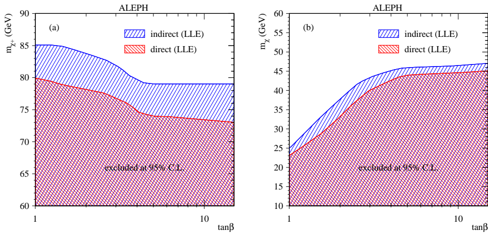
Fig. 5. The 95% C.L. limit on a the chargino mass, b the lightest neutralino mass as a function of \tan\beta , assuming the dominance of either direct or indirect decay modes. The limits hold for any choice of \mu, M_2, m_0 and the generation indices i, j, k of the coupling \lambda_{ijk}
