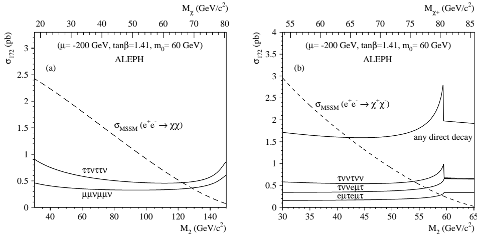
Fig. 6. Cross sections at \sqrt{s} = 172 GeV excluded at 95% C.L. for pair production of a the lightest neutralino and b the lightest chargino, for various final states as a function of M_2 at \tan\beta = 1.41 , m_0 = 60 GeV/ c^2 , \mu = -200 GeV/ c^2 . In b candidates selected at \sqrt{s} = 161 GeV are restricted to m_{\chi^+} < 80.5 GeV/ c^2
