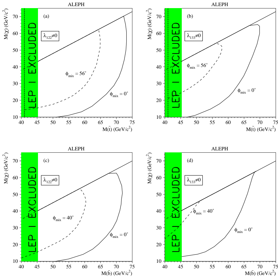
Fig. 12a–d. The 95% C.L. limits on the stop and sbottom in the (m_\chi, m_{\bar{q}}) plane. The two choices of \lambda_{122} and \lambda_{133} correspond to the best and worst case exclusions, respectively. The mass limits are shown for minimal squark mixing ( \phi_{\text{mix}} = 0^\circ ), and for \phi_{\text{mix}} = 56^\circ, 40^\circ for stops and sbottoms, respectively. The LEP 1 limit for \phi_{\text{mix}} = 0^\circ (and \phi_{\text{mix}} = 56^\circ for stops – dashed-dotted lines) is also shown
