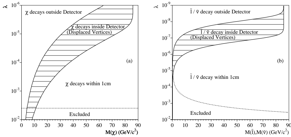
Fig. 2. Regions in the (\tilde{M}, \lambda) -plane where pair-produced LSPs at \sqrt{s} = 172 GeV have a mean decay length of X < 1 cm, 1 \text{ cm} < X < 3 m (displaced vertices), and 3 \text{ m} < X (LSP decays outside detector) for a neutralinos (with M_{\tilde{f}} = 100 \text{ GeV}/c^2 ), b sleptons and sneutrinos. The dashed lines show the low energy limit on \lambda_{133} from (3)
